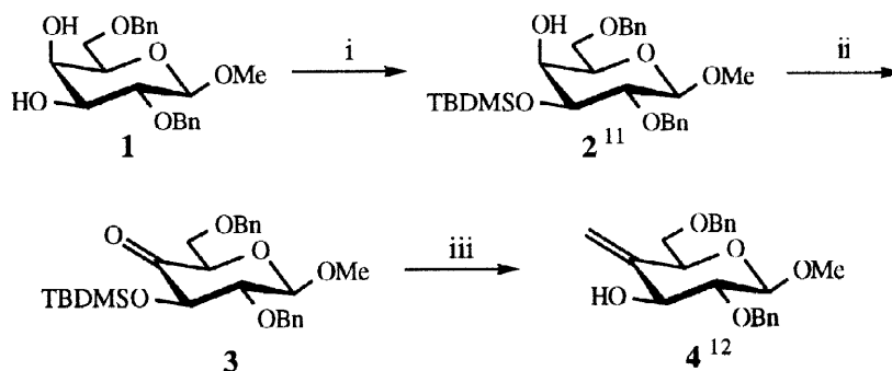
Scheme 1. Reagents. i: TBDMSCl (1.2 equiv), Et 3 N (2 equiv), DMAP (0.4 equiv), DMF, RT, 20h, 96%. ii : PCC (4 equiv), 4Å molecular sieves, CH 2 Cl 2 , RT, 30 min, 85%. iii : 1) Tebbe reagent (2.5 equiv), THF/Pyridine, -60°C \rightarrow RT; 2) aq. HF, THF, RT, 24h, 61%.
